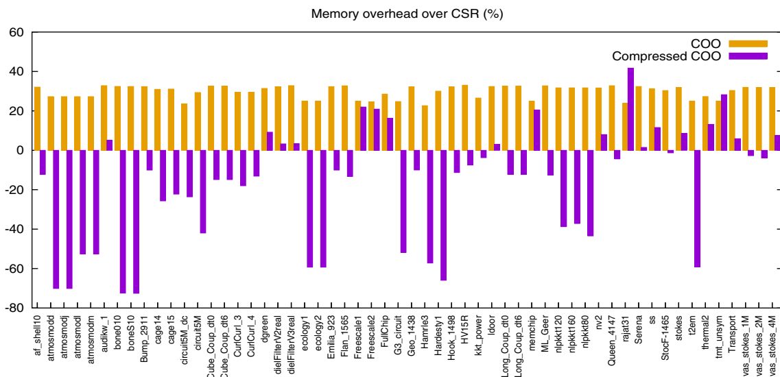
FIGURE 1 Memory overhead of the many-core GPU version of the compressed COO formats taking the CSR format as baseline. All data are assumed to be stored in DP
