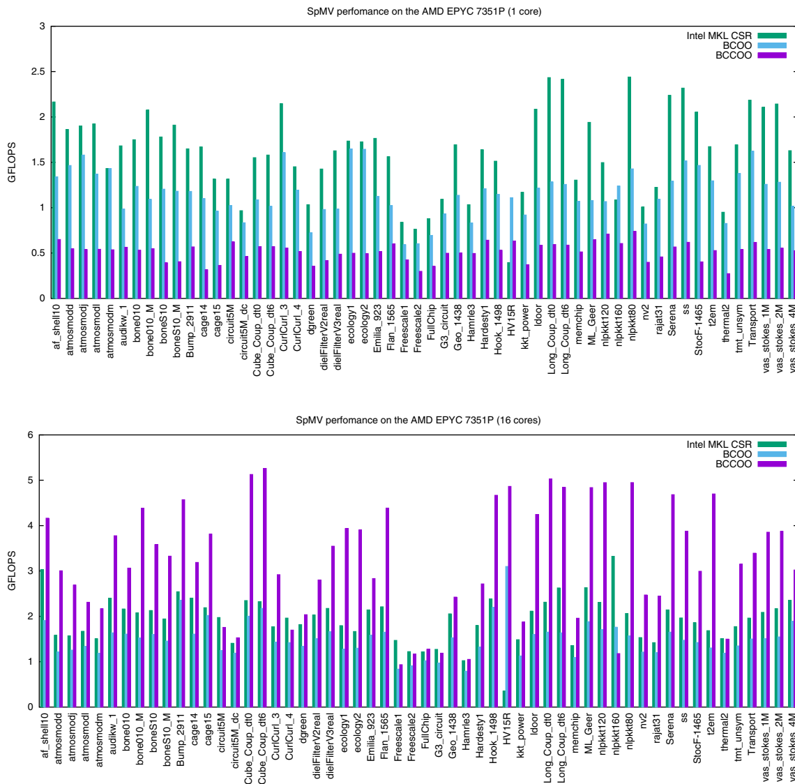
FIGURE 4 Performance of the BCCOO SPMV in comparison with Intel's MKL COO SPMV and Intel's MKL CSR SPMV using 1 core (top) and the full server (1 socket and 16 cores, bottom) of the AMD EPYC 7351P platform
