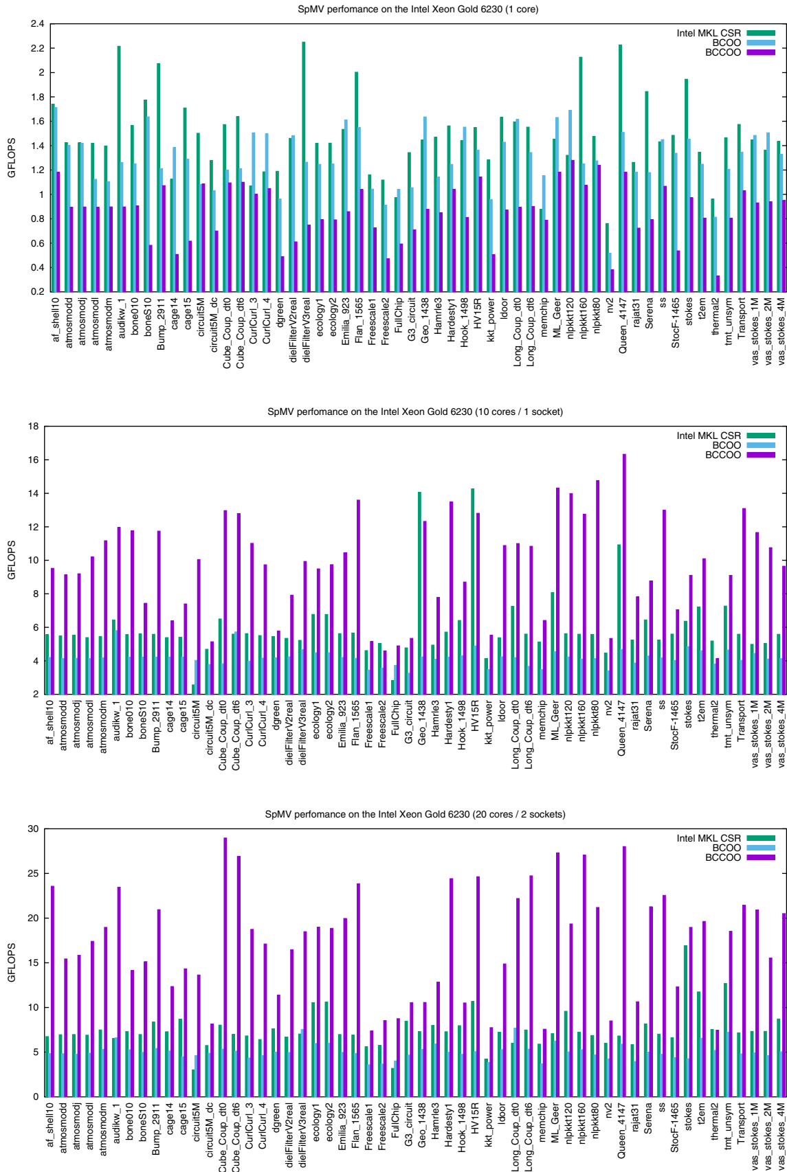
FIGURE 5 Performance of the BCCOO SPMV in comparison with Intel's MKL COO SPMV and Intel's MKL CSR SPMV using 1 core (top), a single socket (10 cores, center), and the full server (2 sockets and 20 cores, bottom) of the Intel Xeon Gold 6230 platform
