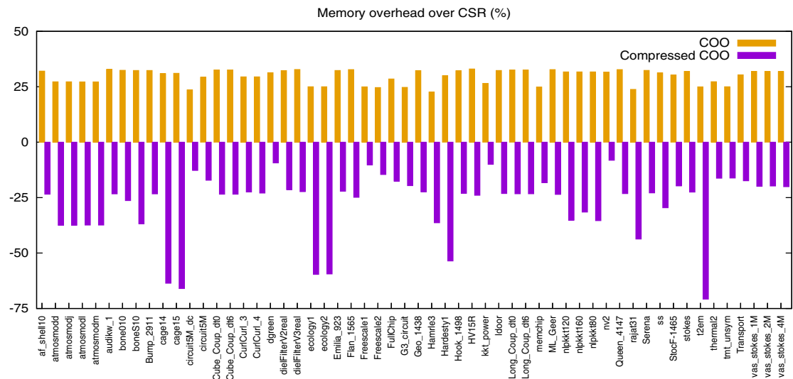
FIGURE 3 Memory overhead of the multicore CPU version of the compressed COO format taking the CSR format as baseline. All data are assumed to be stored in DP
