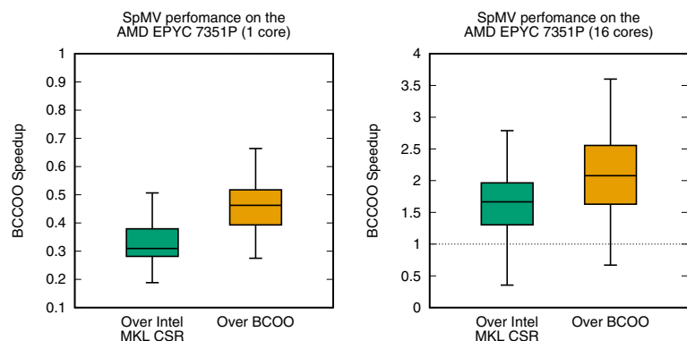
FIGURE 7 Speedup analysis comparing the performance of the BCCOO SPMV against Intel's CSR SPMV and the BCOO SPMV on the AMD EPYC 7351P
