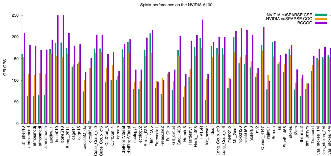
FIGURE 2 Performance of the BCCOO SPMV in comparison to the cuSPARSE COO SPMV and the cuSPARSE CSR SPMV on NVIDIA V100 (top) and A100 (bottom) GPUs
