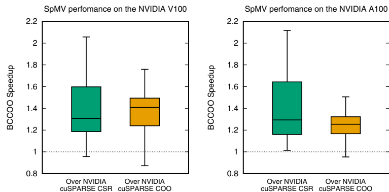
FIGURE 6 Speedup analysis comparing the performance of the BCCOO SPMV against the COO SPMV and the CSR SPMV from NVIDIA's cuSPARSE library on the NVIDIA V100 (left) and NVIDIA A100 (right)
