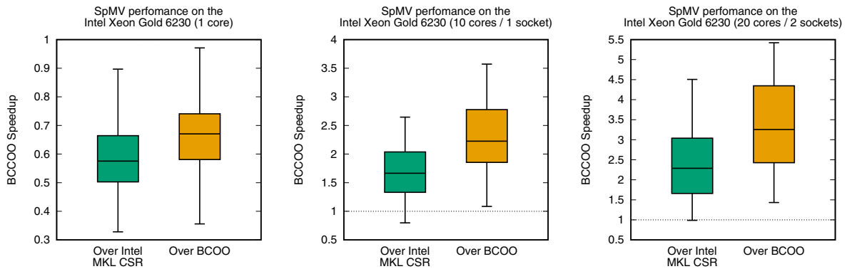
FIGURE 8 Speedup analysis comparing the performance of the BCCOO SPMV against Intel's CSR SPMV and the BCOO SPMV on the Intel Xeon Gold 6230
