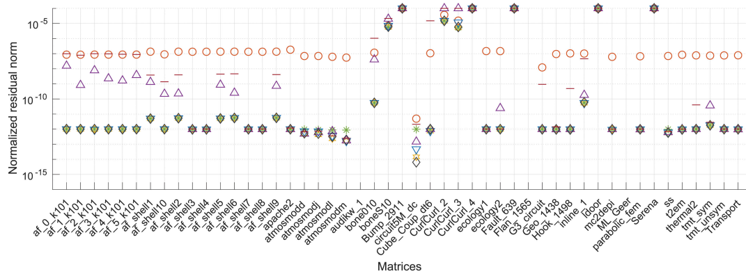
Figure 11. Normalized residual of ILU-preconditioned GMRES and ILU-preconditioned CB-GMRES using different precision for arithmetic and memory operations.
