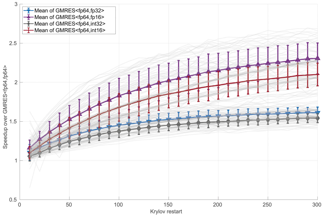
Figure 9. Speed-up for different CB-GMRES variants (GMRES<arith,mem>) over DP GMRES (GMRES<fp64,fp64>) for increasing restart values.
