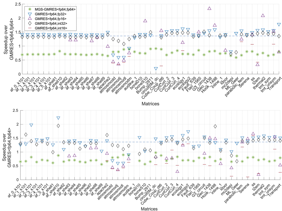
Figure 8. Speed-up of the non-preconditioned CB-GMRES (top) and Jacobi-preconditioned CB-GMRES
