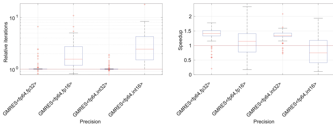
Figure 7. Statistics obtained from running the CB-GMRES algorithms on the 49 test problems. Left: iteration overhead (relative to DP GMRES) and right: speed-up relative to DP GMRES. The data reflects both the non-preconditioned runs and the Jacobi-preconditioned settings.
