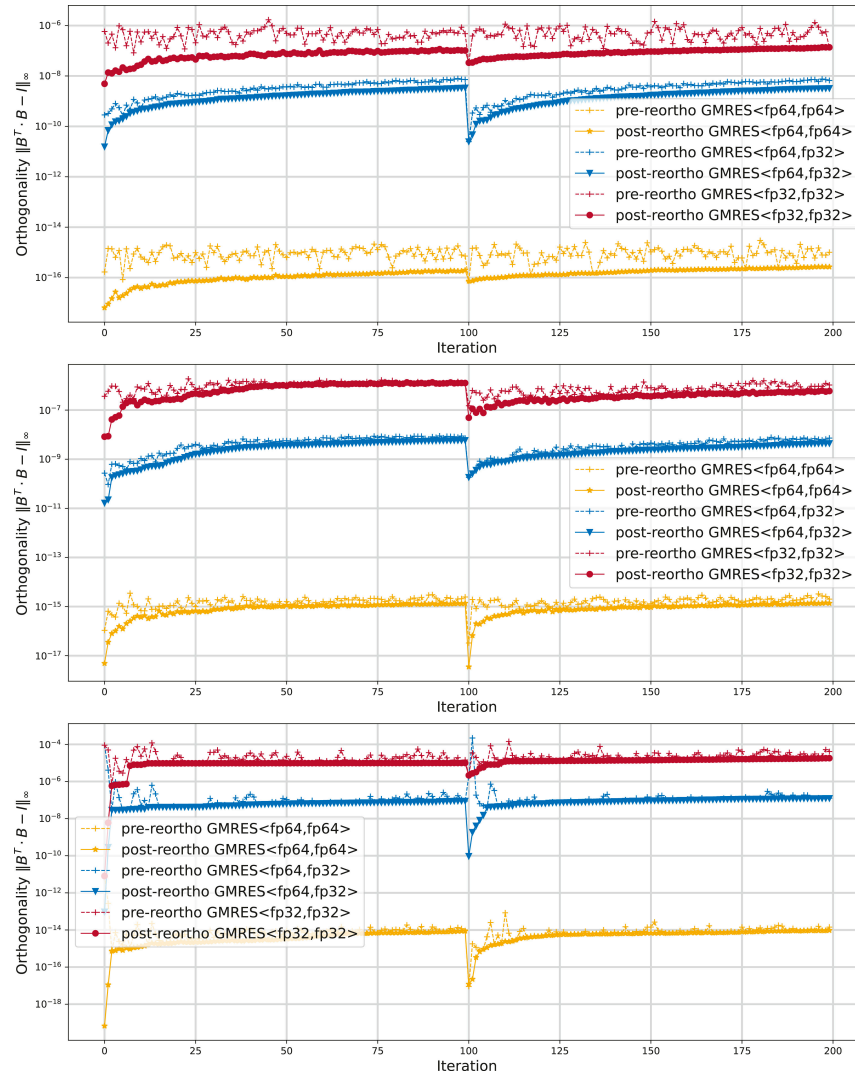
Figure 3. Orthogonality of the Krylov basis vectors before and after re-orthogonalization for the standard DP GMRES and SP GMRES and the CB-GMRES GMRES<fp64,fp32>. The test matrices are parabolic_fem (top), ss (center), and circuit5M_dc (bottom).
