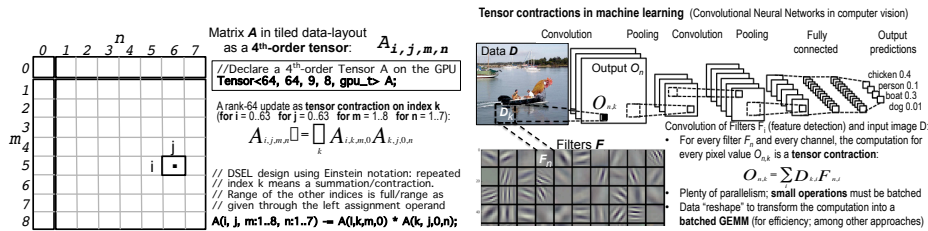
Figure 1: Left: Example of a 4 th -order tensor contractions design using Einstein summation notation and a domain-specific embedded language ( DSEL ). Right: Illustration of batched computations needed in machine learning.
