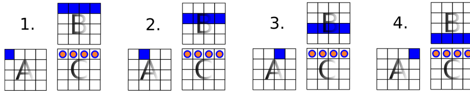
Figure 5: Computing the first row of C in a 4-by-4 matrix product using SIMD.
