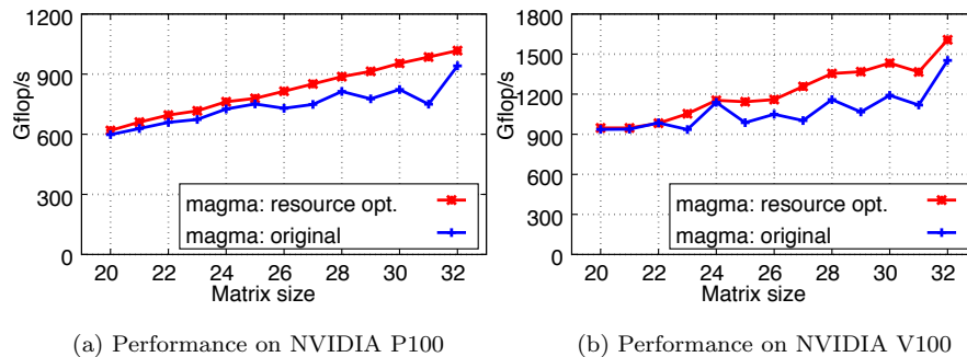
Figure 16: Impact of resource optimization on performance. The experiment is performing 100,000 GEMM operations in double precision.
