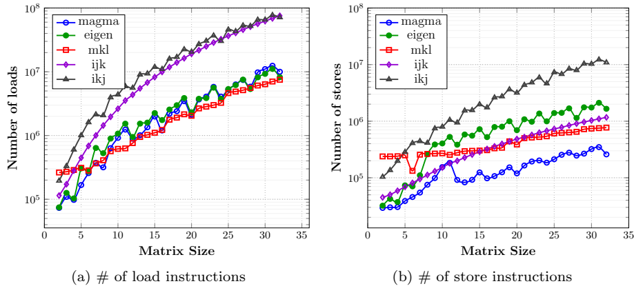
Figure 7: CPU Performance counters measurement of the memory accesses on Intel Xeon E5-2650 v3 processor (e.g., Haswell).
