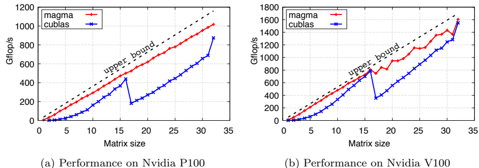
Figure 18: Final obtained performance of 100,000 GEMM operations in double precision on a Tesla P100 and V100 GPU.
