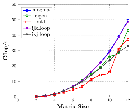
(c) Performance on sizes up to 12
