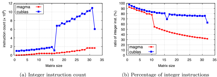
Figure 17: Profiling the instruction mix of MAGMA versus CUBLAS. The experiment is performing 100,000 GEMM operations in double precision on a Tesla P100 GPU.
