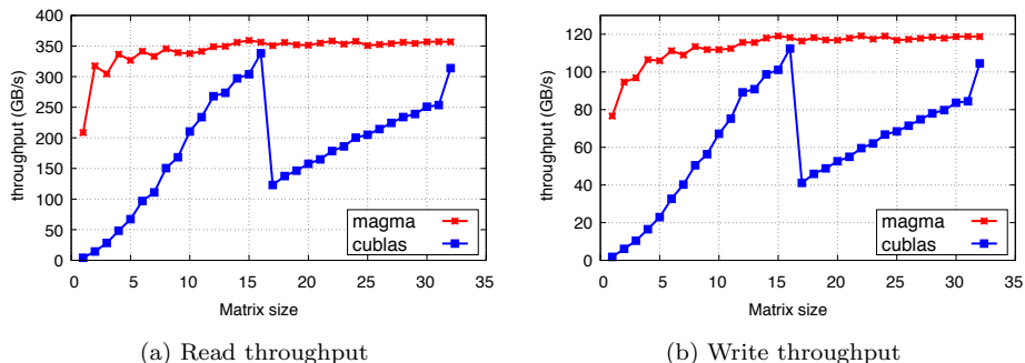
Figure 20: DRAM read and write throughputs. The experiment is performing 100,000 GEMM operations in double precision on a Tesla P100 GPU.
