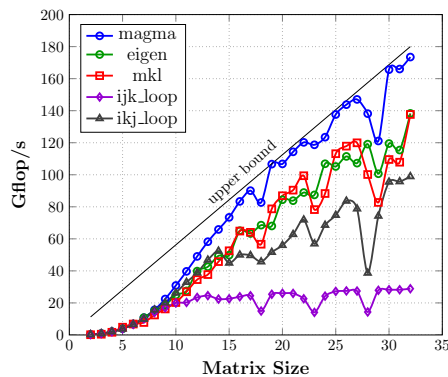
(a) CPU performance comparison without MCDRAM
