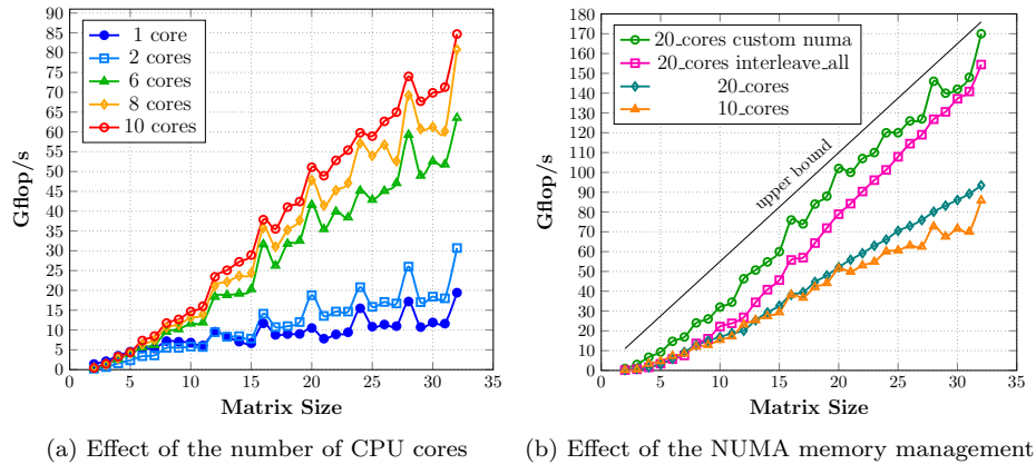
Figure 9: CPU Performance analysis on Haswell.
