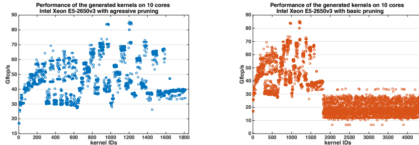
(a) Tuning of the dgemm kernel using the aggressive pruning strategy. (b) Tuning of the dgemm kernel using the basic hardware constraint pruning.
