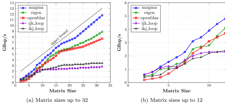
Figure 13: Experimental results of the matrix-matrix multiplication on the Tegra X1.
