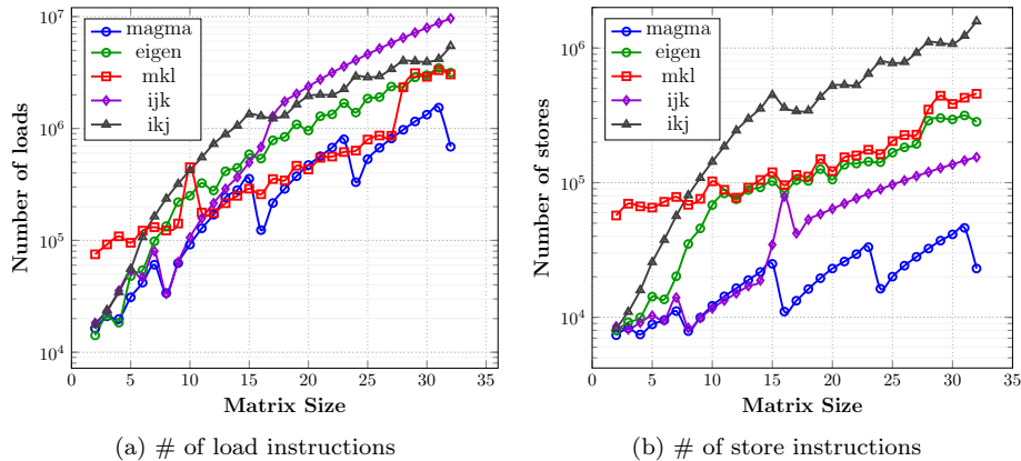
Figure 10: CPU performance counters measurement of the memory accesses on KNL.
