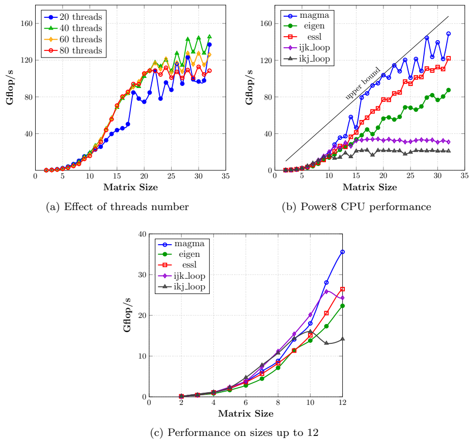
Figure 14: Experimental results of the matrix-matrix multiplication on a POWER8 processor.
