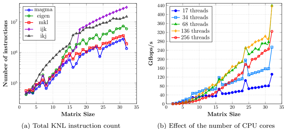
Figure 11: CPU performance counters and scaling analysis on KNL.
