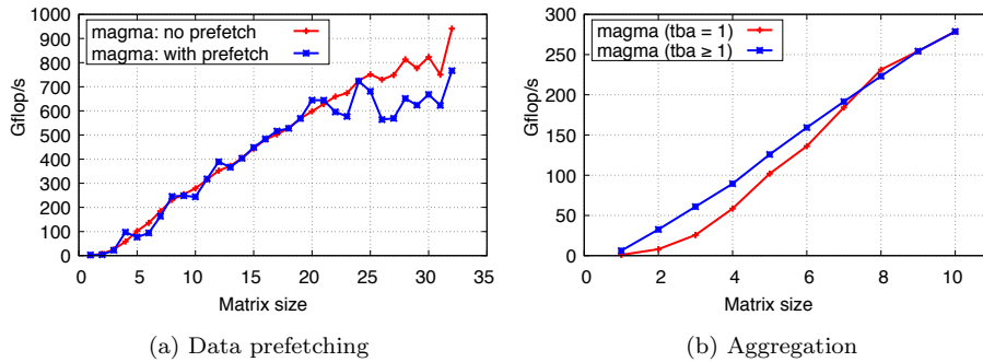
Figure 15: Impact of data prefetching and aggregation on performance. The experiment is performing 100,000 GEMM operations in double precision on a Tesla P100 GPU.
