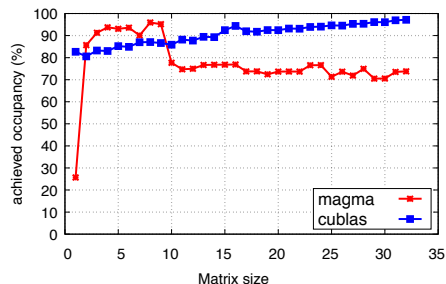
Figure 19: Profiling the achieved occupancy of MAGMA versus cuBLAS. The experiment is performing 100,000 GEMM operations in double precision on a Tesla P100 GPU.
