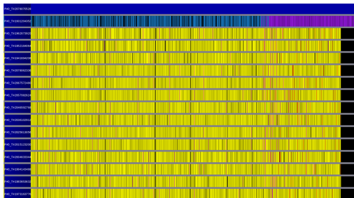
Fig. 6. OOM Tile QR algorithm: Trace of the optimized left looking panel update and factorize.
