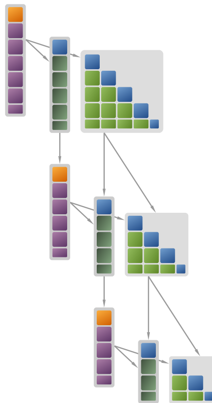
Figure 2.6: Dynamic tasking.
