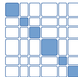
Figure 2.4: Rectangular tiling.
