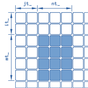
Figure 2.5: Matrix dimensions.
