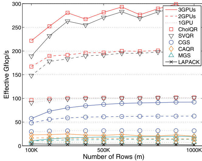
FIG. 4. Performance of standard TSQR implementations in double precision with up to three NVIDIA Tesla M2090 GPUs. “LAPACK” uses DGEQRF and DORGQR of threaded MKL on 16-core Intel SandyBridge CPU, and “effective Gflop/s” is computed as the ratio of the total flops required by DGEQRF and DORGQR for the same input matrix over the orthogonalization time, in seconds. The number of columns is fixed at 30 (i.e., n = 30 ).
