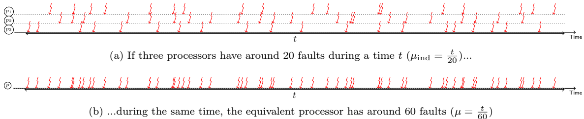
Figure 7: Intuition of the proof of Proposition 1.
