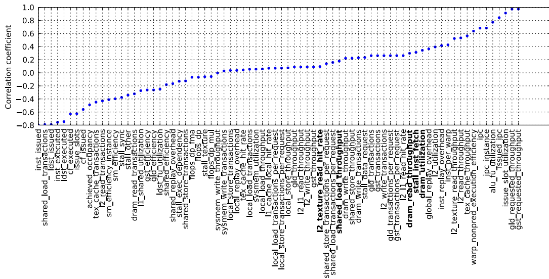
Figure 8. Correlation coefficients of the collected performance metrics and the GFLOPs value.
