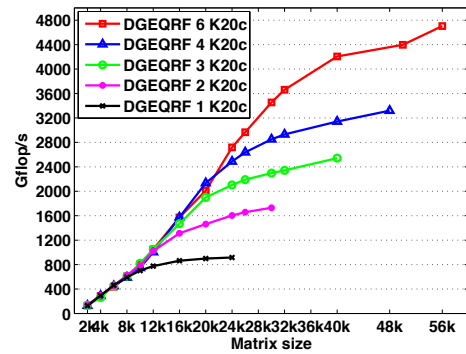
Figure 13: Performance scalability of the QR decomposition on multicore CPU and multiple accelerators (up to 6 Kepler K20c).
