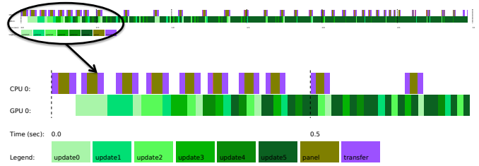
Figure 4: Trace of the Cholesky factorization on multicore 16 Sandy Bridge CPU and a K20c GPU, using priorities to improve lookahead.
