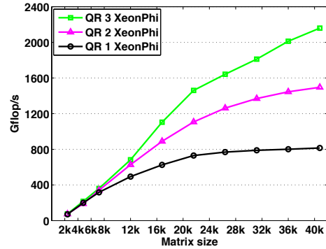
Figure 14: Performance scalability of the QR decomposition on multicore CPU and multiple accelerators (up to 3 Xeon Phi).
