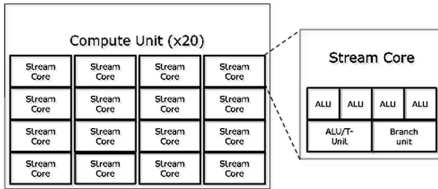
Fig. 6. Radeon 5870 architecture.
