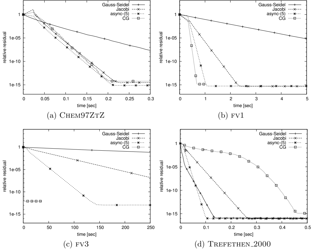
Figure 9: Relative residual behavior with respect to solver runtime.
