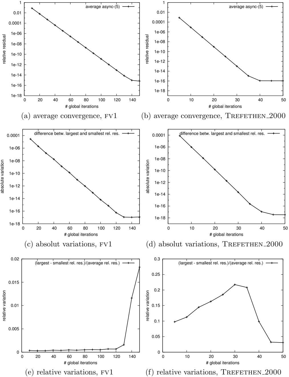
Figure 5: Visualizing the average convergence, the absolute respectively relative variations in the convergence behavior of async-(5) depending on the number of conducted global iterations.
