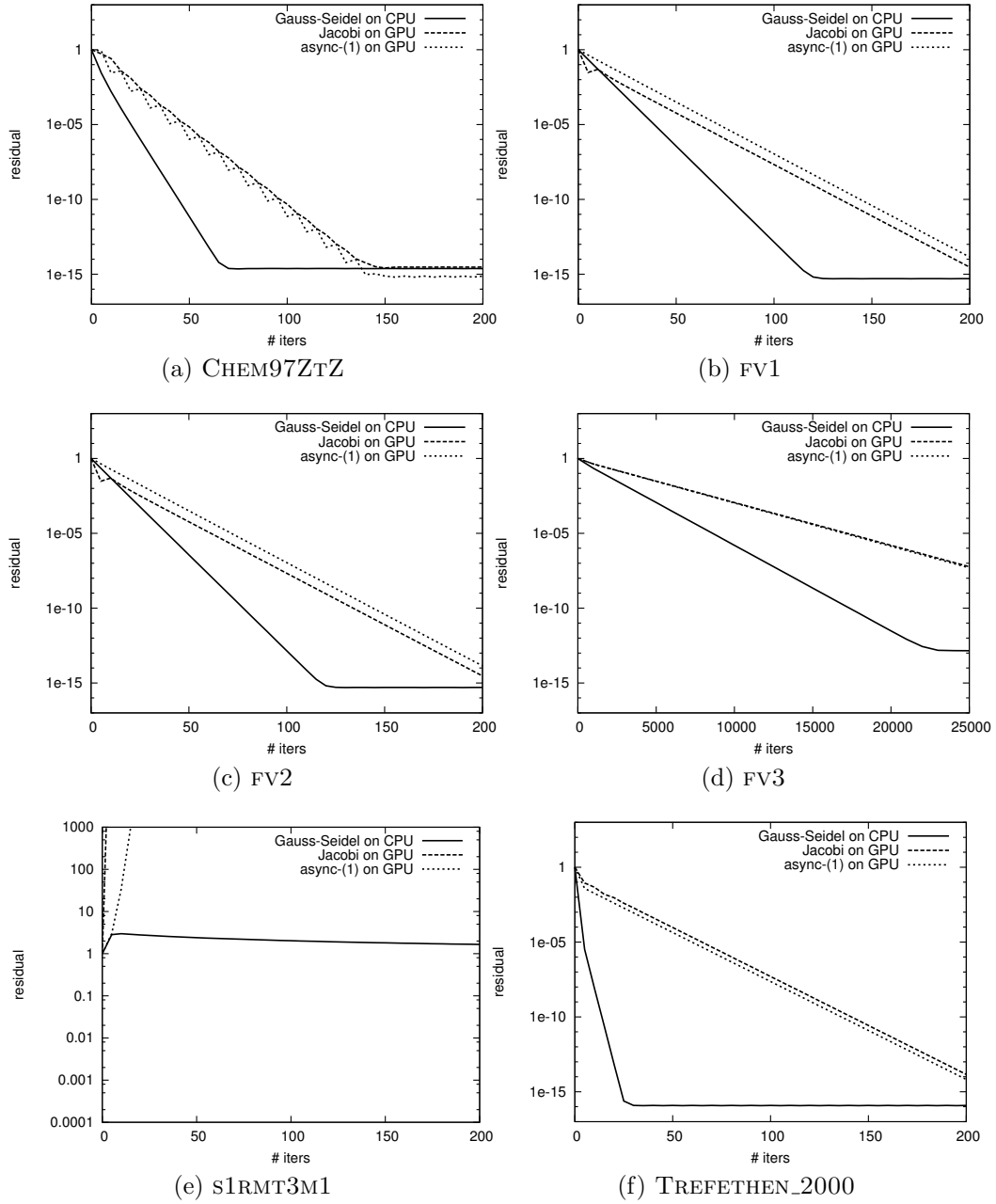
Figure 6: Convergence behavior for different test matrices.
