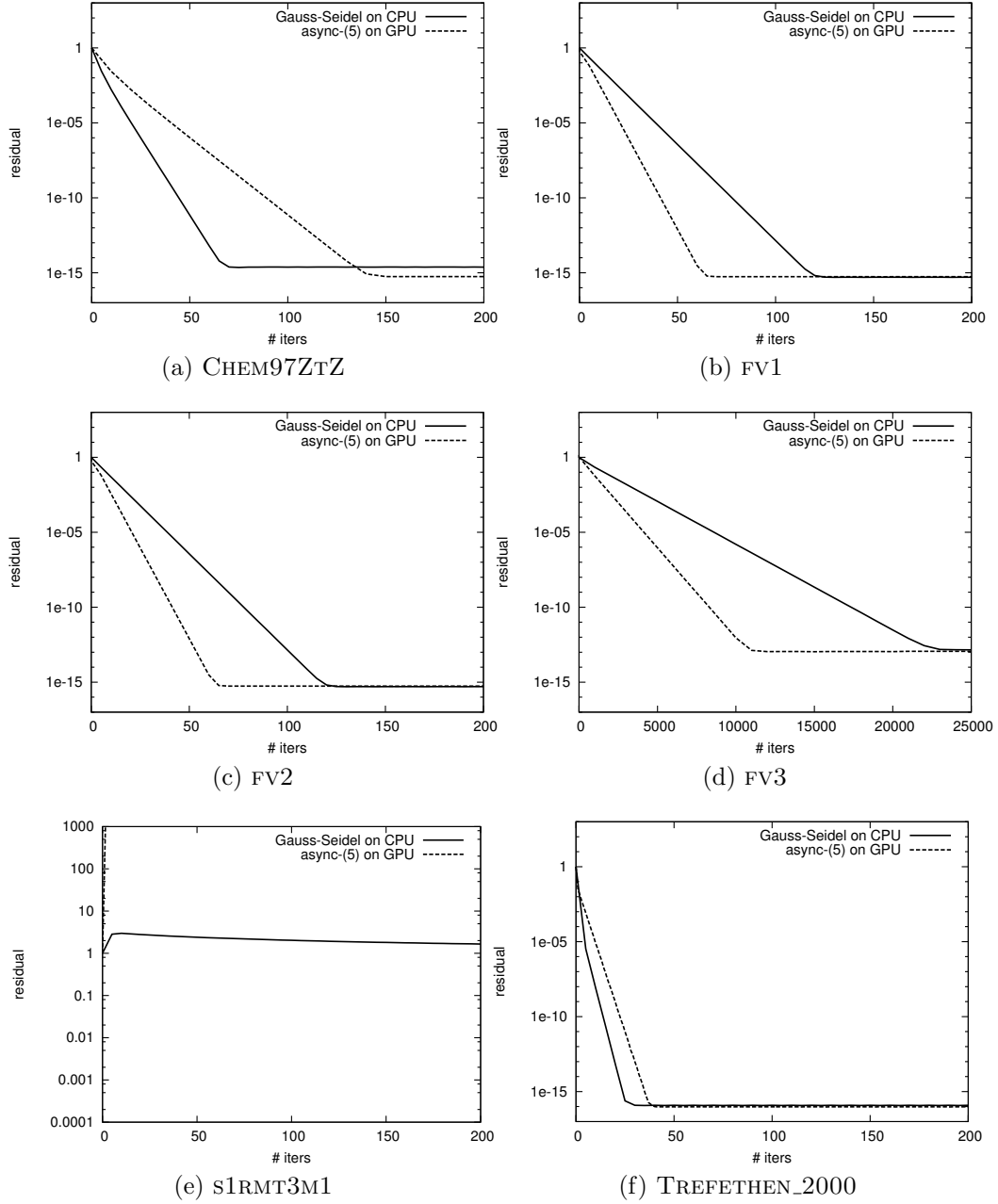
Figure 7: Convergence rate of block-asynchronous iteration.
