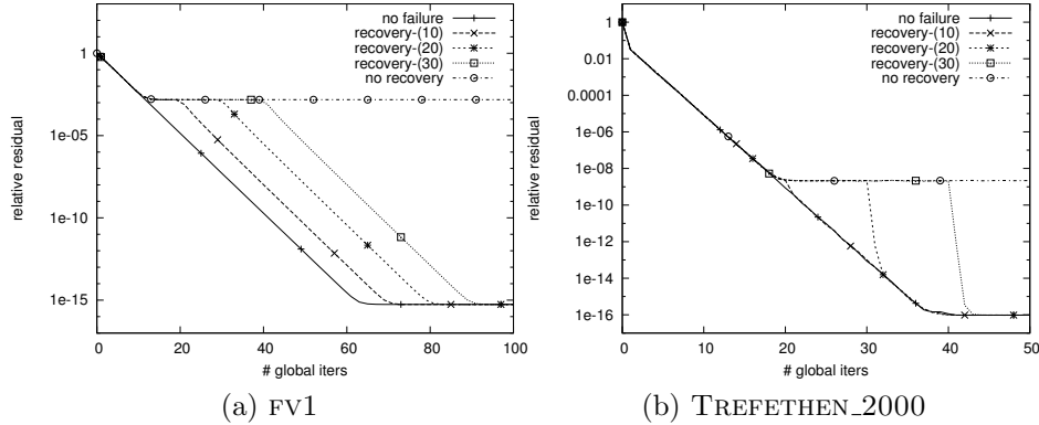
Figure 10: Convergence of async-(5) for hardware failure. The implementations either recover by reassigning the components to other cores after the recovery time t_r (denoted with recover-( t_r ) ), or generate a solution approximation with significant residual error.
