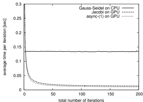
Figure 8: Average iteration timings of CPU/GPU implementations depending on total iteration number, test matrix FV3.
