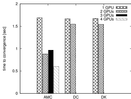
Figure 11: Time-to-solution for the different Multi-GPU implementations for test matrix TREFETHEN_20000.
