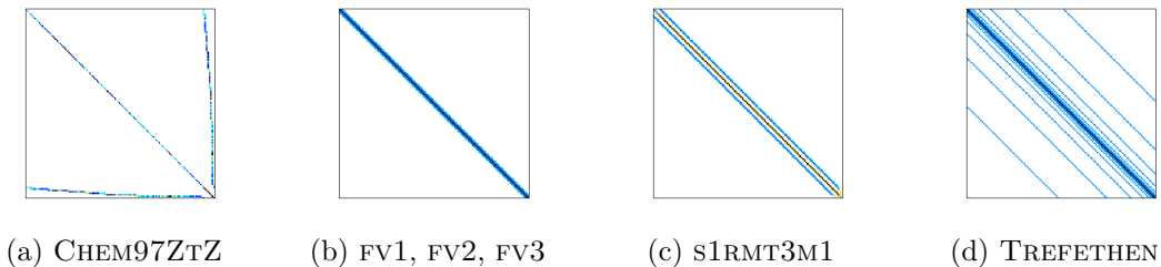
Figure 1: Sparsity plots of test matrices.
