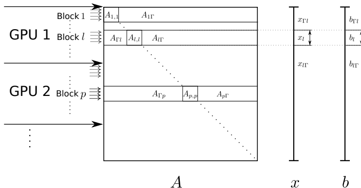
Figure 3: Visualizing the block-asynchronous iteration for multi-GPU implementation.
