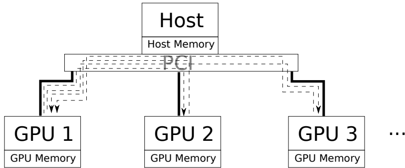
(b) GPU-direct memory transfer ( DC ), GPU1 serves as master-GPU.
