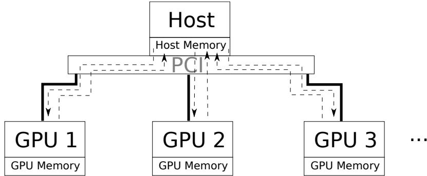
(a) Asynchronous multicopy ( AMC )
