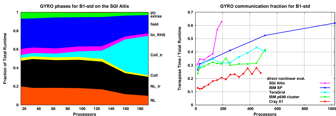
Figure 2. Phase diagram for B1-std on the SGI Altix and inter-platform comparison of time spent in transpose events
