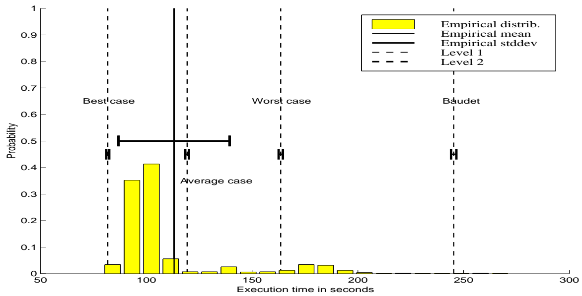
Figure 9: Experiment vs. Characterization for the first asynchronous implementation
