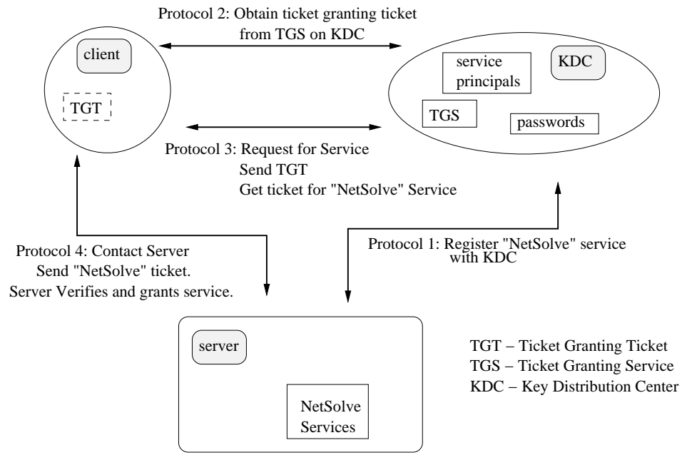
Figure 3: NetSolve/Kerberos Interaction: A NetSolve server "registers" its services with the KDC, which authenticates clients wanting to use that service within NetSolve. The NetSolve server becomes a Kerberos service and the NetSolve client becomes a Kerberos client as well.
